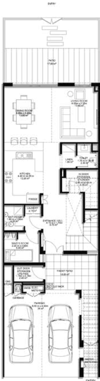
Ground Floor
