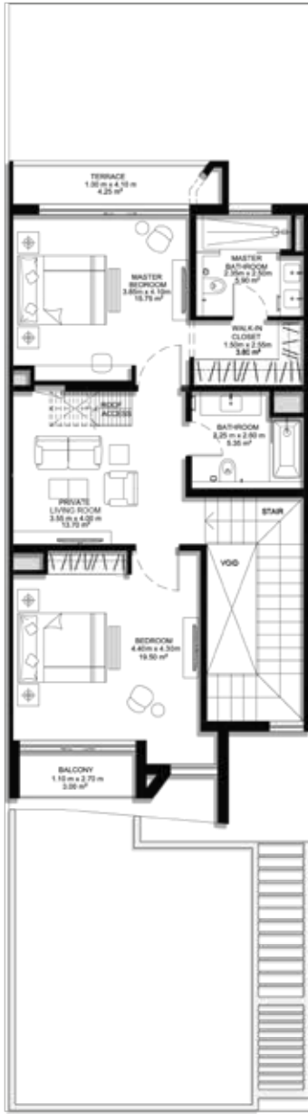
First Floor
