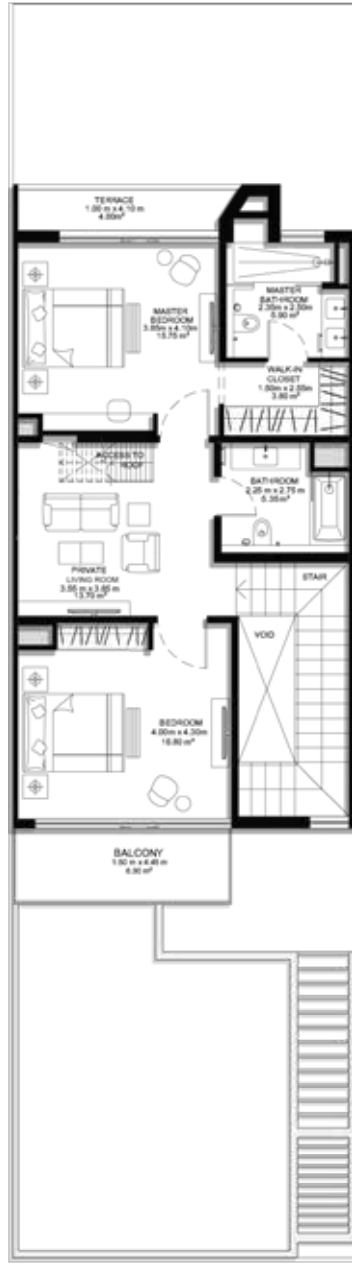
First Floor
